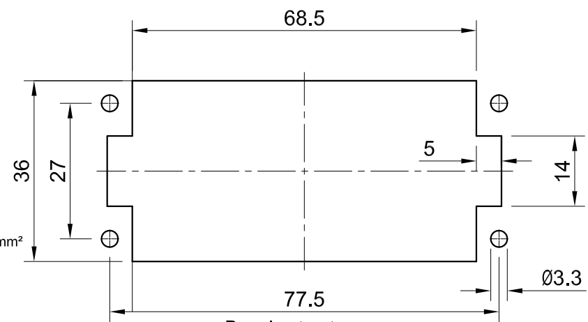
Panel cut out 面板开孔尺寸
